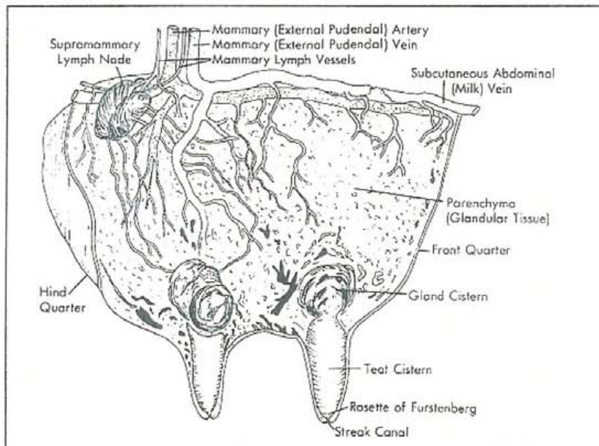
Components of udder showing blood supply (Frandsen, 1986)
