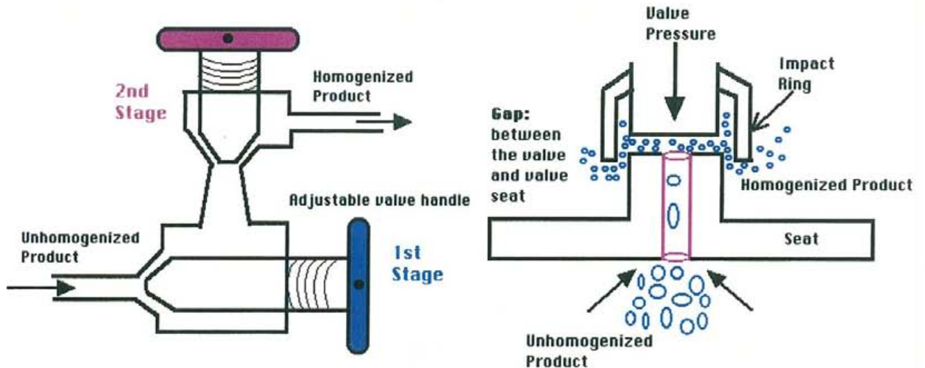
Homogenizer and Valve
