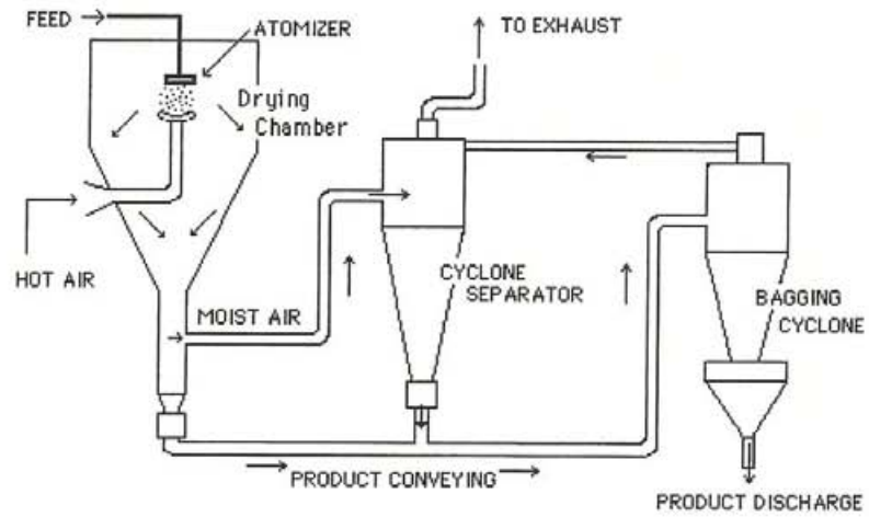
Cyclone Dryer
