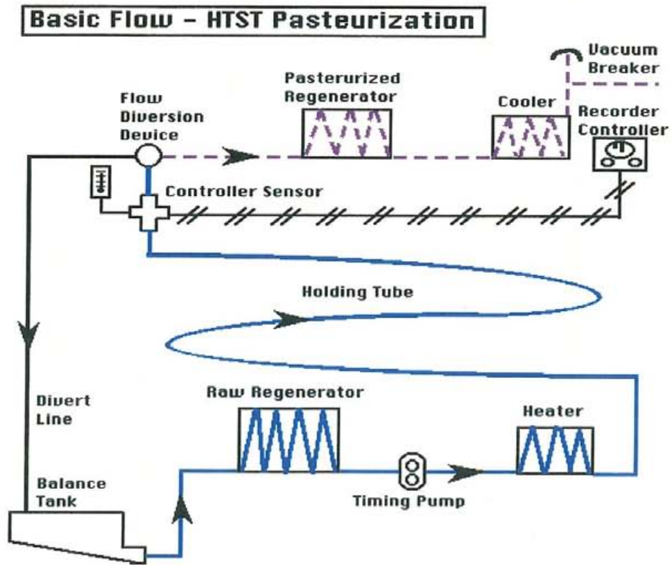
HTST milk pasteurization equipment and the flow of milk through it [ http://www.foodsci.uoguelph.ca/dairyedu/pasteurization.html ]
